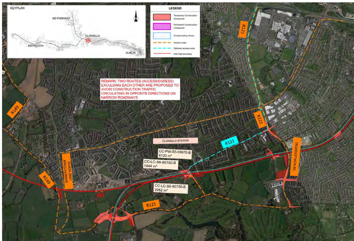
Figure 5-277 Clonsilla permanent way compound haulage route
