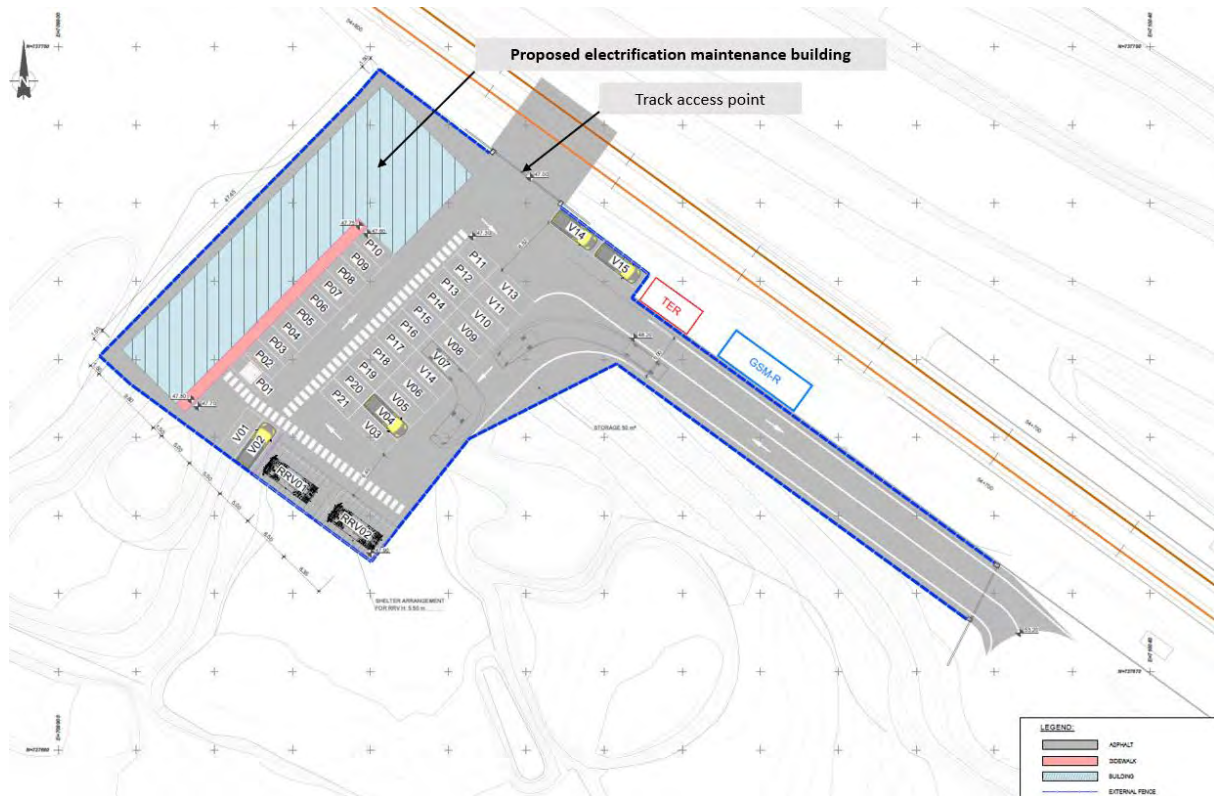
Figure 5-246 Navan Road permanent maintenance compound
