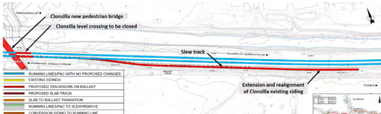
Figure 5-275 Location of Clonsilla siding
