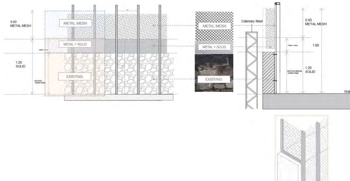
Figure 5-93 Design intent for parapet heightening on walls
