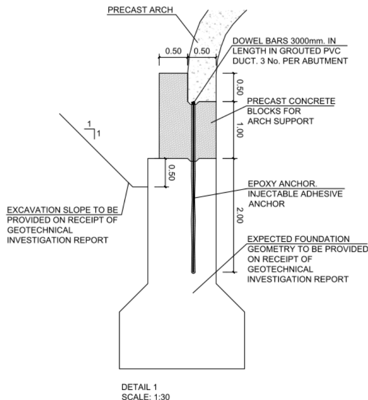
Figure 5-46 Connection detail between between existing foundation and new precast wall block
