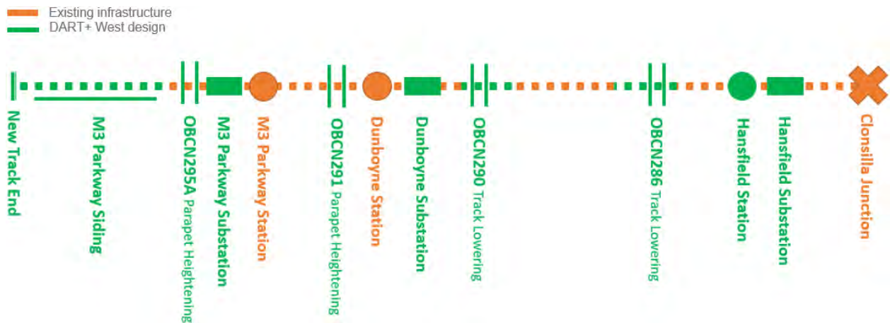
Figure 5-281 Schematic of DART+ West construction activities in Zone D
