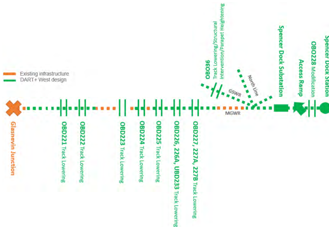
Figure 5-128 Schematic of DART+ West construction activities in Zone B
