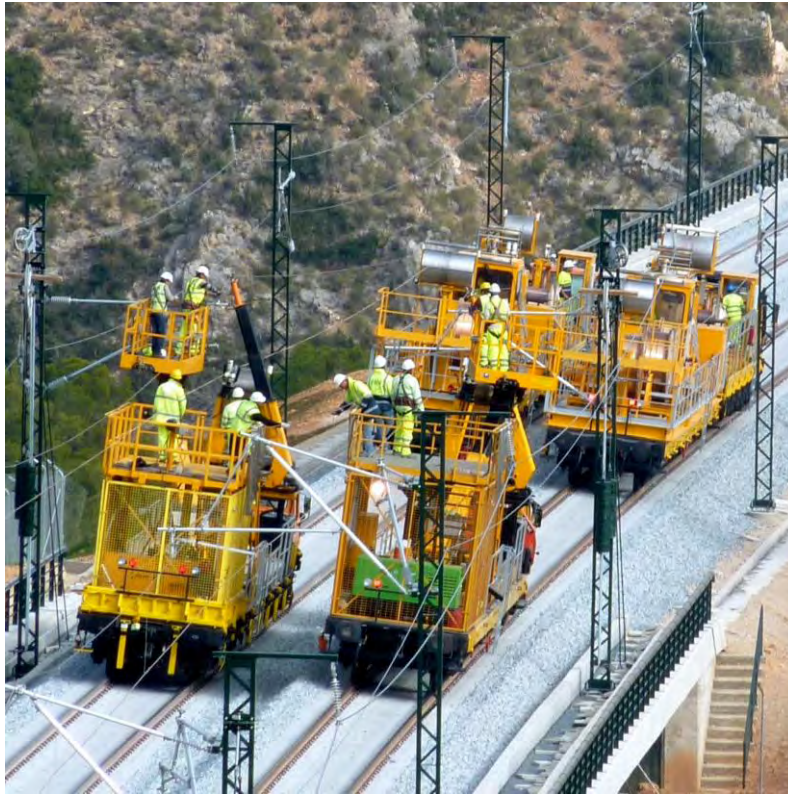
Figure 5-85 Wire installation track vehicles
