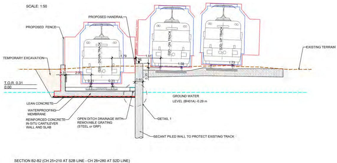
Figure 5-193 Structure B - section B2-B2
