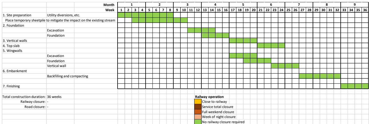
Figure 5-365 Construction duration of UBG22B
