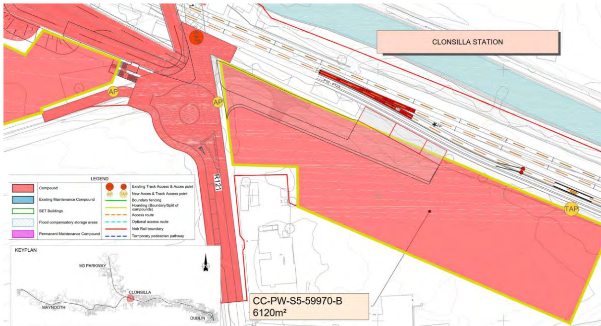
Figure 5-276 Clonsilla permanent way compound
