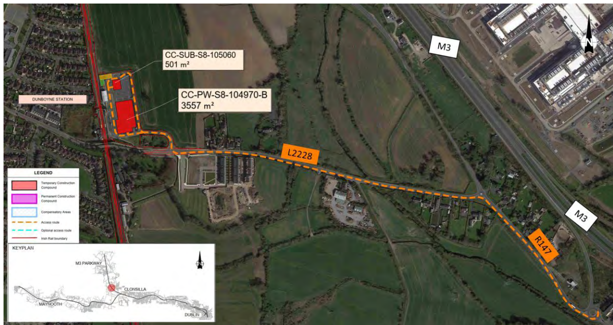
Figure 5-288 Dunboyne permanent way compound and haulage route
