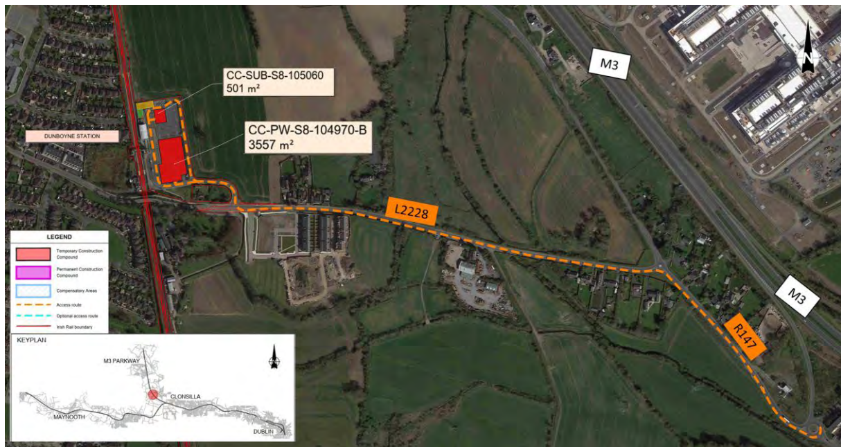
Figure 5-290 Dunboyne substation compound and haulage route
