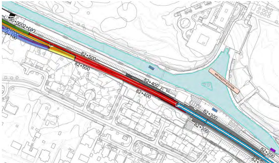
Figure 5-354 Maynooth station track realignment & crossover replacement (red)
