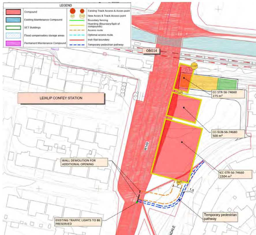
Figure 5-317 Leixlip Confev substation compound
