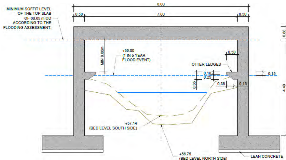
Figure 5-363 Cross section of UBG22B
