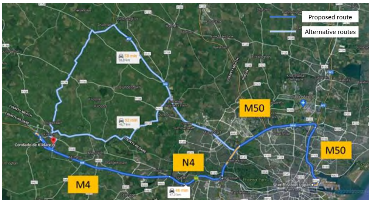
Figure 5-165 Route for transport of spoil material from Spencer Dock to depot
