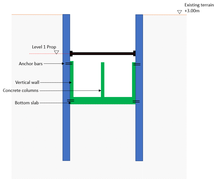
Figure 5-180 Phase 7 – construction of tank walls and columns
