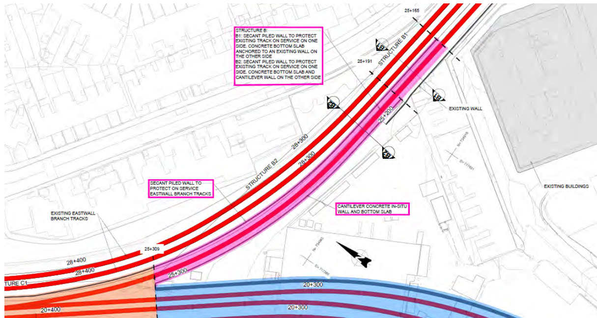
Figure 5-192 Spencer Dock proposed walls and protection slabs - Structure B
