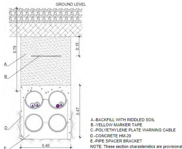
Figure 5-42 Example of buried PVC ducts
