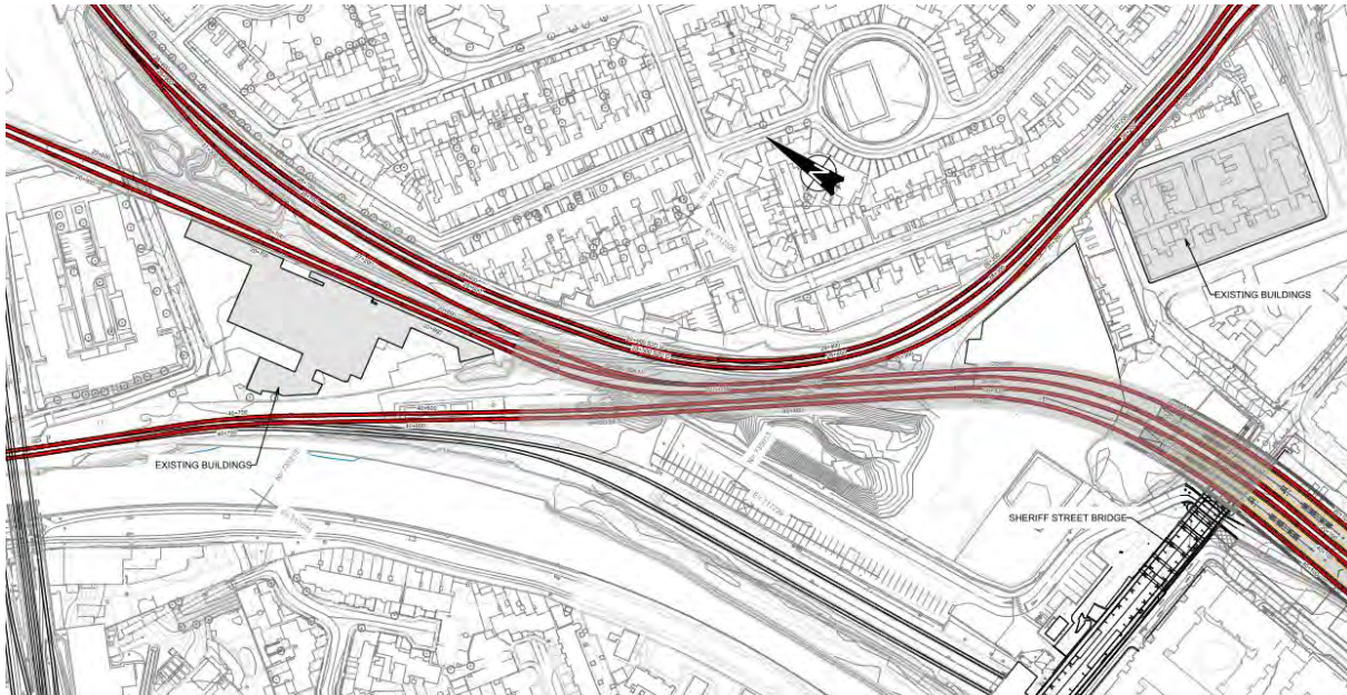
Figure 5-188 Spencer Dock proposed track alignment
