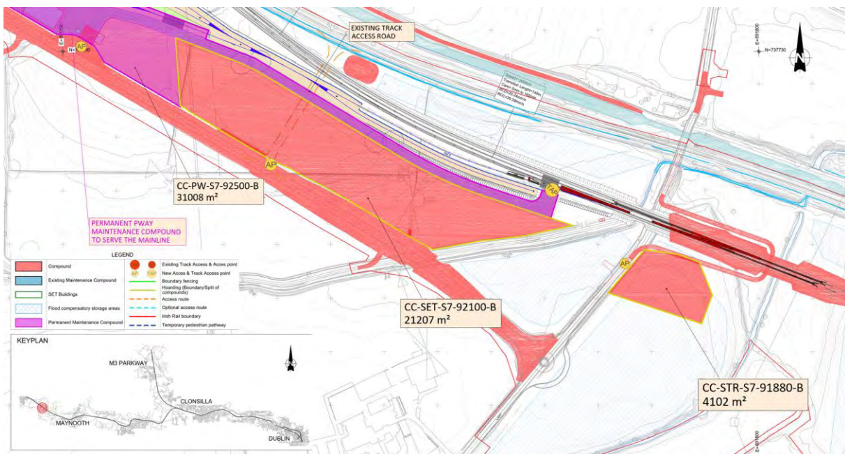
Figure 5-367 Millfarm structures compound
