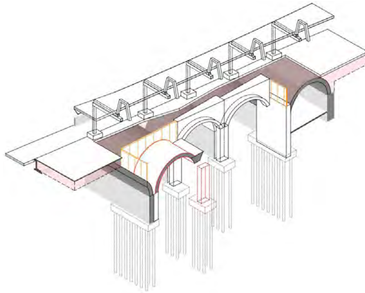
Figure 5-108 3D view of step 7 – arched slab construction
