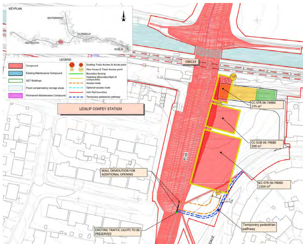
Figure 5-313 OBG14 structures compound
