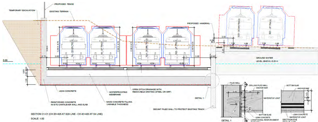
Figure 5-196 Structure C – section C1-C1
