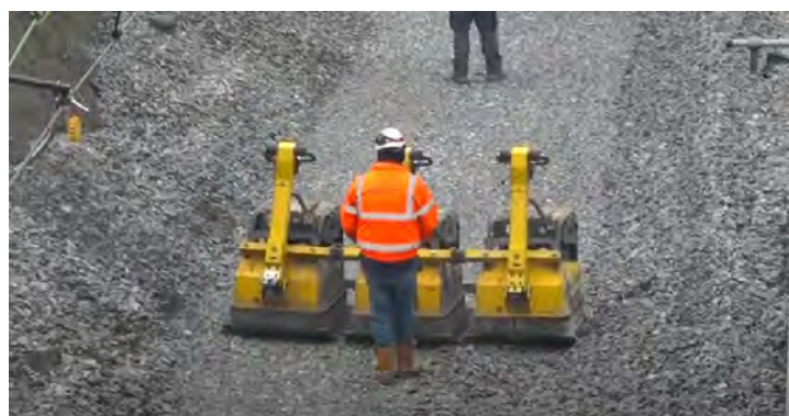
Figure 5-18 Ballast compaction
