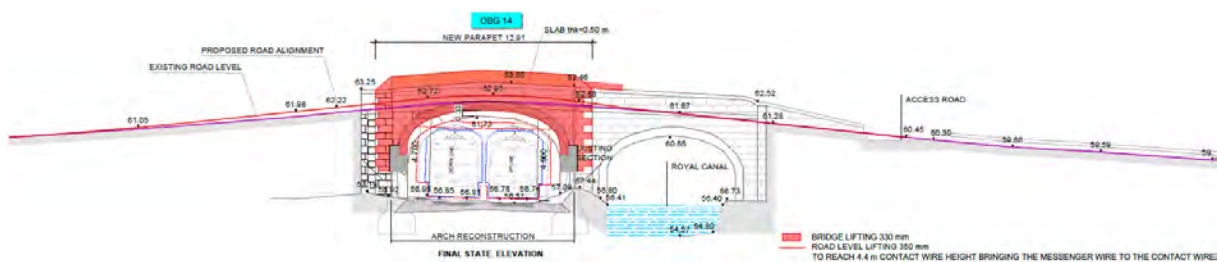
Figure 5-305 Elevation of OBG14 deck reconstruction
