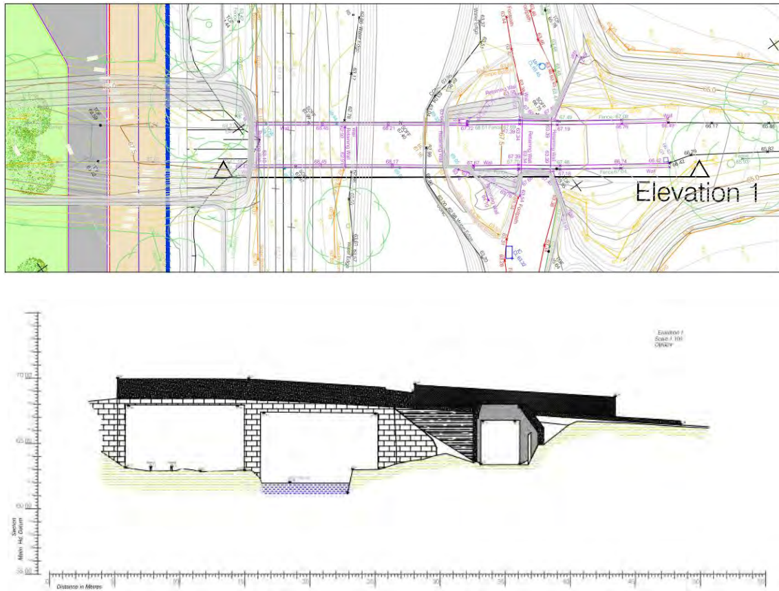
Figure 5-388 Plan (above) and elevation (below) of OBG24 (bridge and underpass for Royal Canal greenway)
