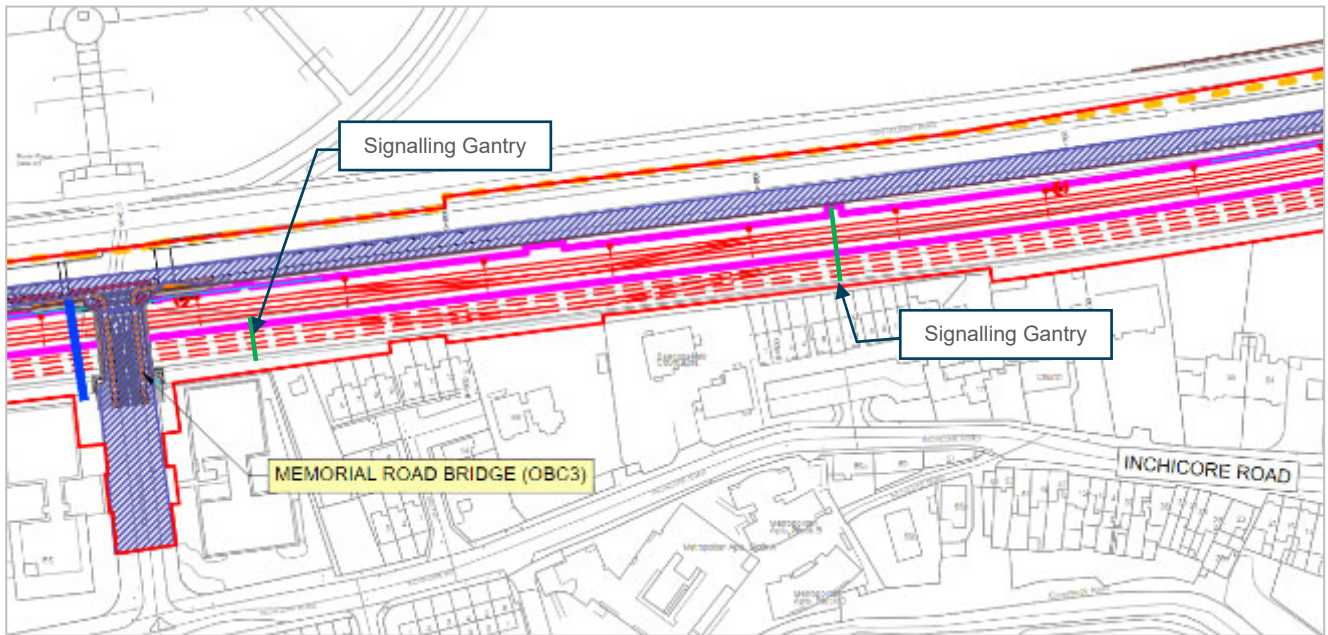
Figure 4-97 New Signalling Cantilevers (Chainage 9+780 and 9+970)
