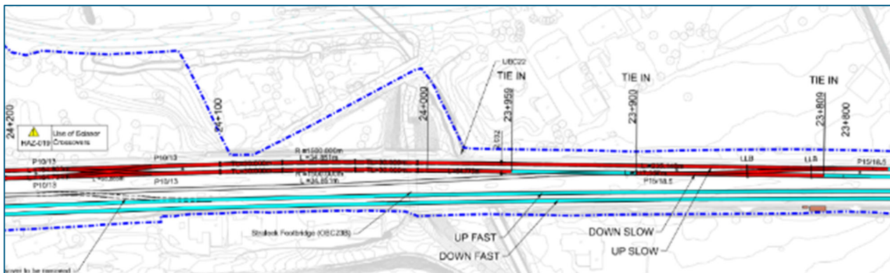
Figure 4-27 Hazelhatch & Celbridge Station – Track Plan Layout (3 of 3)
