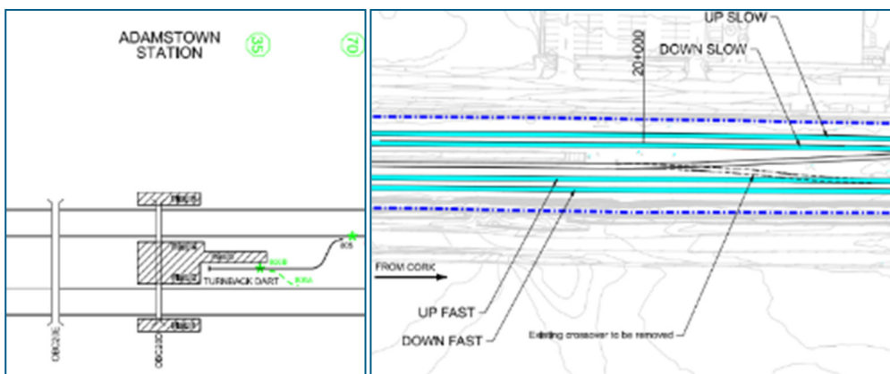
Figure 4-28 Adamstown Station- Track Plan Layout (1 of 2)
